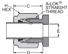
A-LOK® Double Ferrule Fitting
