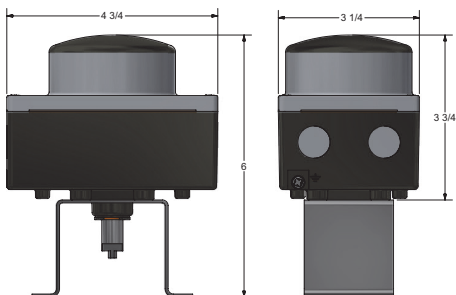
SB Limit Switch
