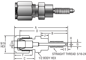
Calibration Adapter for Rosemount/Foxboro DP Transmitters
