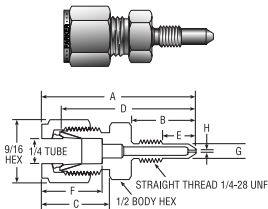
Calibration Adapter for Honeywell DP Transmitters
