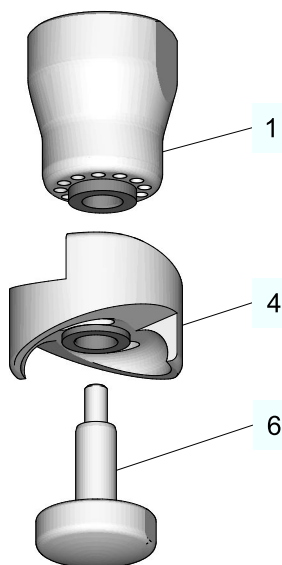
Fig.9: Rotor with cap
