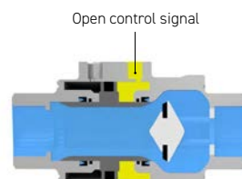
Piloted state (valve open)
